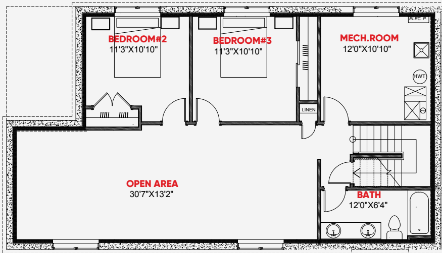
BASEMENT FLOOR PLAN 982 sq.ft.
